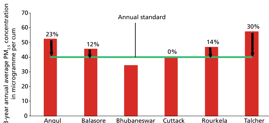
Graph 2: Reduction targets of PM2.5 concentration in six cities
